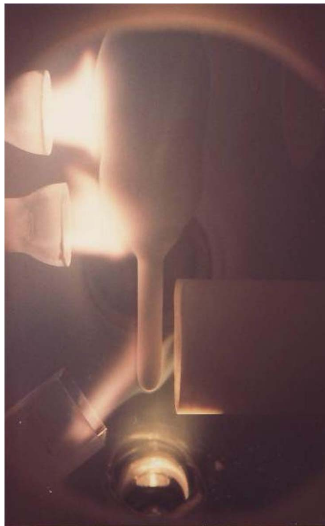
Photograph of multiple torches configuration for VAD single-mode-fiber preform
