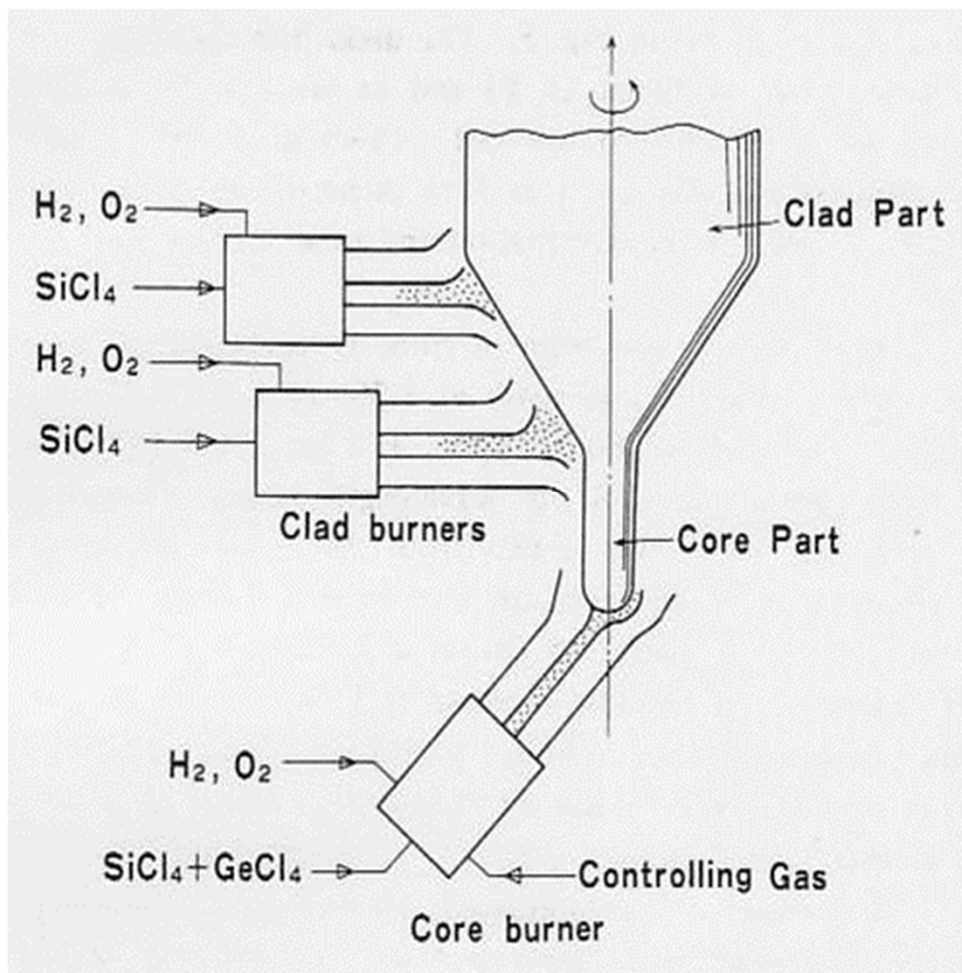
Schematic illustrating multiple torches configuration
